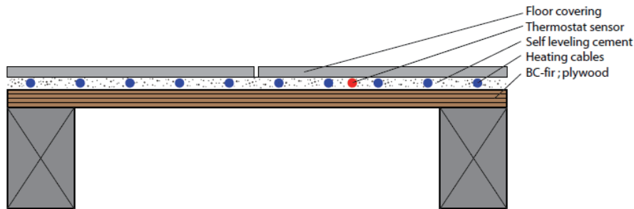
Installation on BC-fir; plywood
